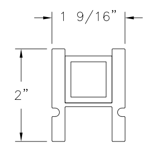
ACTIVE/FIXED PANEL H-REINFORCEMENT ALUMINUM 6063-T5
